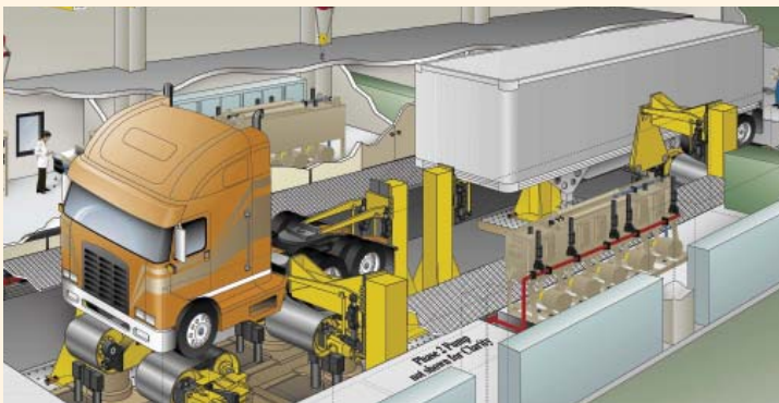
The final phase of the Roadway Simulator will enable testing of tractor-trailer combination vehicles as heavy as forty tons
